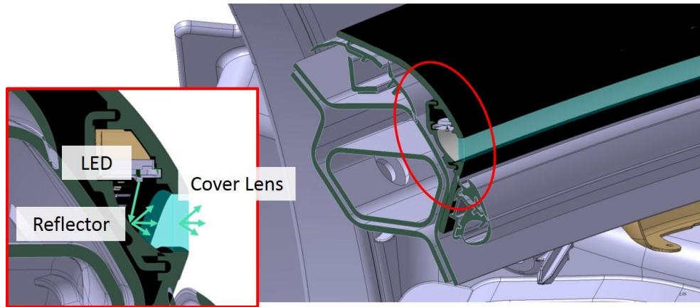
Figure 4: Concept of Light Band at minimal construction spaces.
