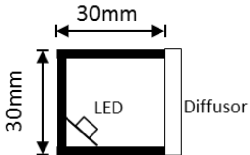
Figure 13: Sketch of the LED stripe (left), bended diffuser for side elements (right).
